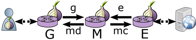
Fig. 1. Measuring positions in a circuit: relay G in position g measures relay M , relay M in position mc measures relay E , relay M in position md measures relay G , and relay E in position e measures relay M . A dashed arrow indicates hosts between which traffic is not measured.
