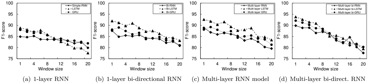
Fig. 7. Performance of authorship verification models with different architectures and RNN units. Notice that the performance enhances with bidirectional RNN and with more depth. All percentage are F1-score.
